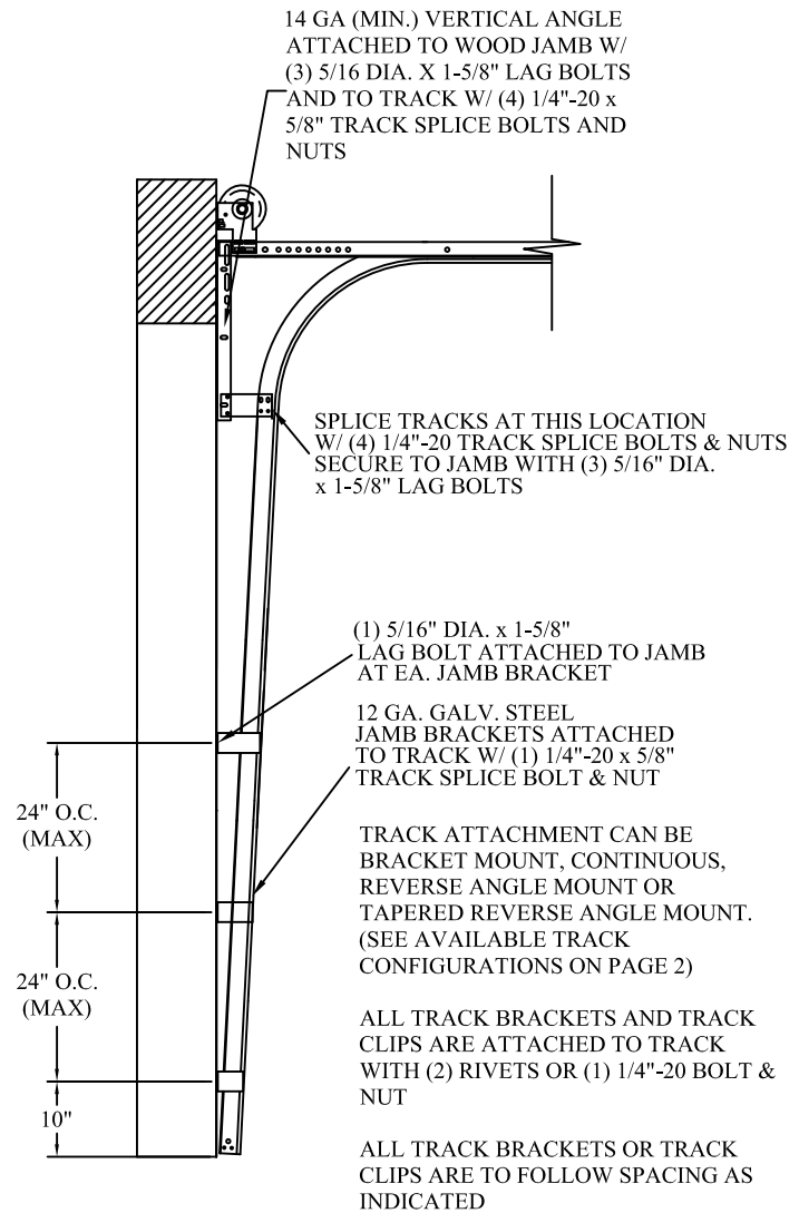
TRACK CONFIGURATION FOR UP TO 24' TALL DOORS N.T.S.
